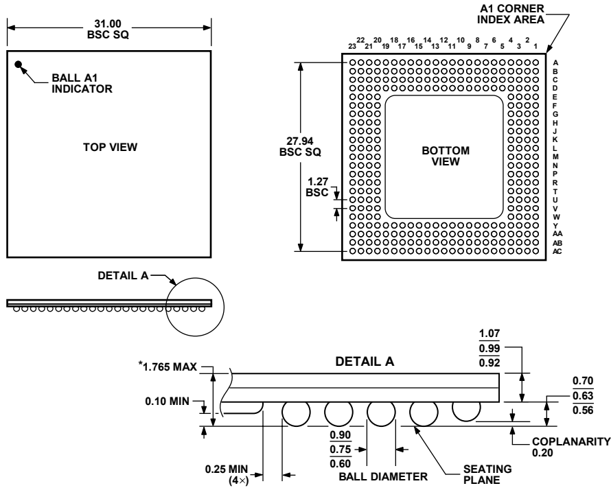
*COMPLIANT TO JEDEC STANDARDS MO-192-BAN-2 WITH THE EXCEPTION TO PACKAGE HEIGHT. Figure 74. 304-Ball Ball Grid Array, Thermally Enhanced [BGA_ED] (BP-304) Dimensions shown in millimeters
